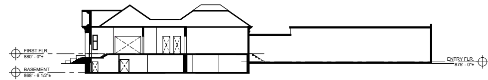
BUILDING SECTION
