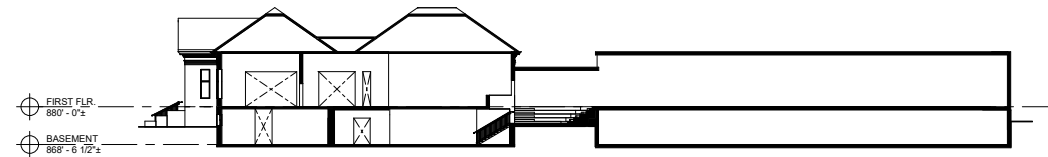
BUILDING SECTION
